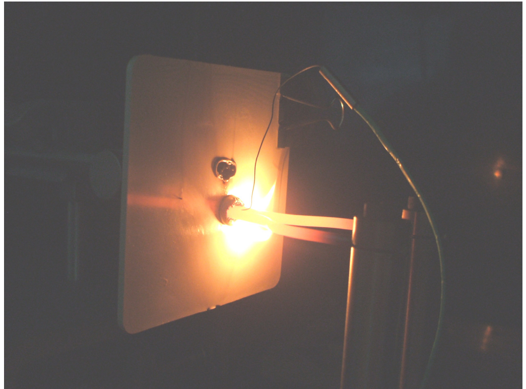
Glow-wire test specimen
