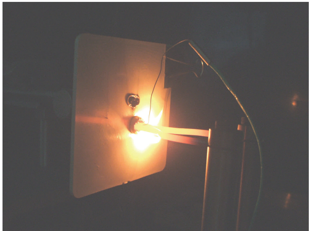
Glow-wire test specimen
